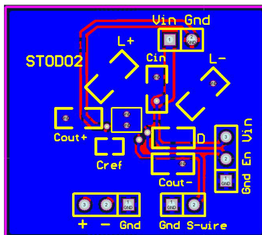
Figure 21. Suggested demonstration board schematic (bottom layer view)
