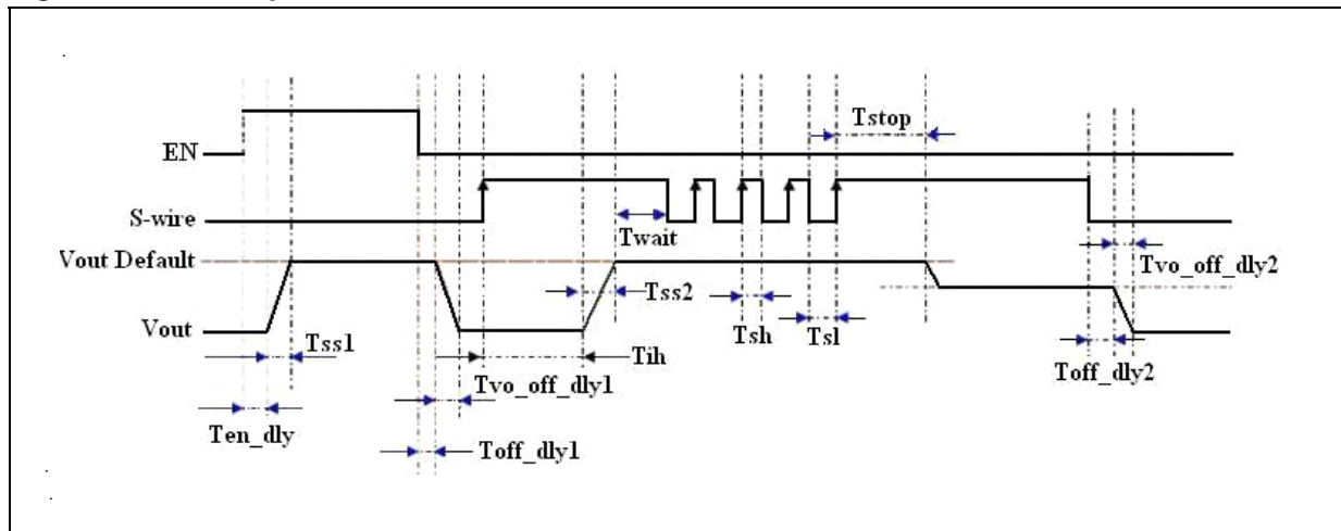
Figure 4. S-wire protocol
