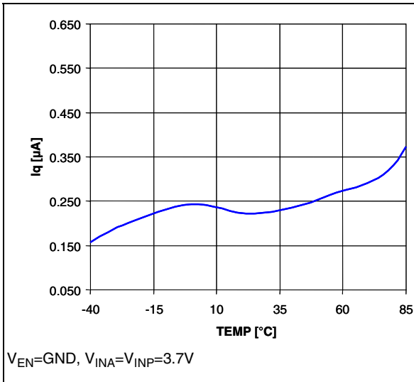
Figure 13. Quiescent current vs. temperature
