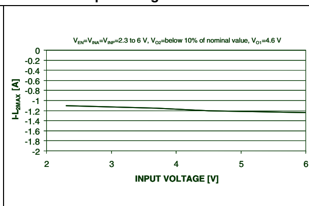
Figure 10. Inverting inductor peak current vs. input voltage
