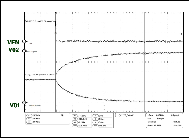
Figure 19. Fast discharge
