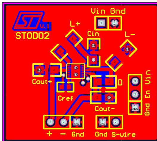
Figure 20. Suggested demonstration board schematic (top layer view)
